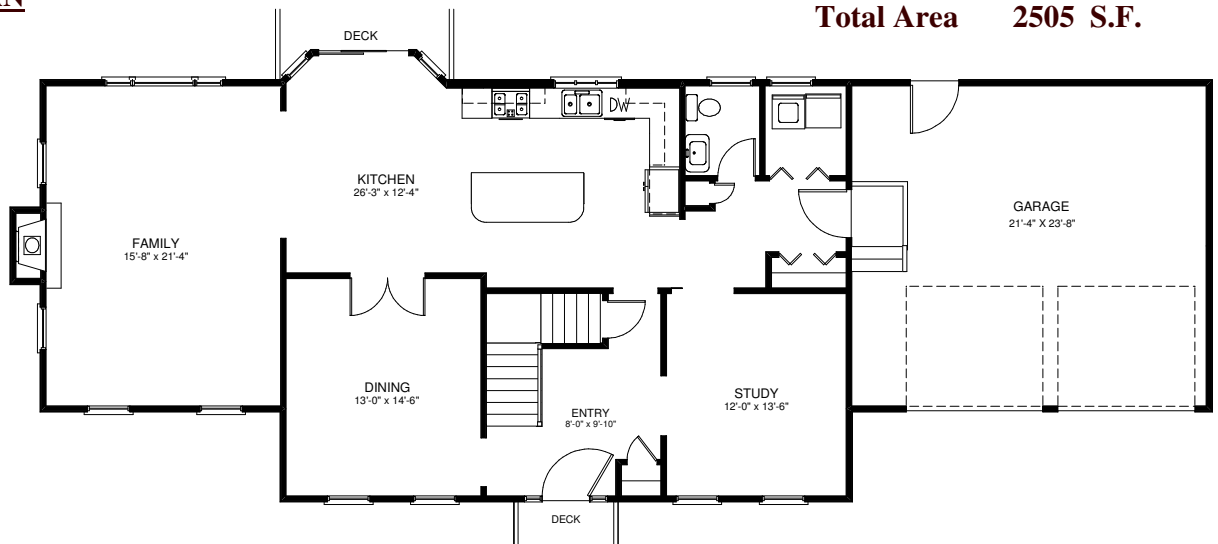
ENTRY LEVEL PLAN
